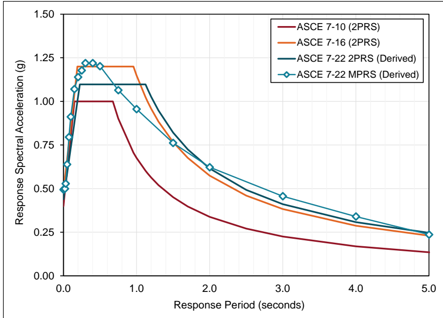
Figure 8.2-4 Comparison of two-period design response spectra (2PRS) of ASCE 7-10, ASCE 7-16, and ASCE 7-22 (as proposed), and multi-period design response spectra (MPRS) of ASCE 7-22 (as proposed) derived from values of S_s , S_l , and T_L using the methods of this study, for the Anchorage (AK) Site assuming Default site conditions.
