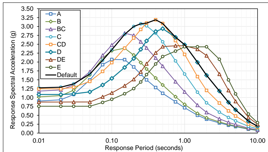
Figure E.2-21 Plots of deterministic MCE_R multi-period response spectra (MPRS) derived from parameters S_S and S_I in accordance with the methods of Chapter 5, Santa Rosa Site.
