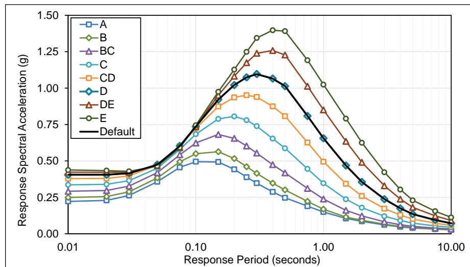
Figure E.1-15 Plots of probabilistic MCE_R multi-period response spectra (MPRS) derived from parameters S_s , S_l , T_L in accordance with the methods of Chapter 4, Sacramento Site.
