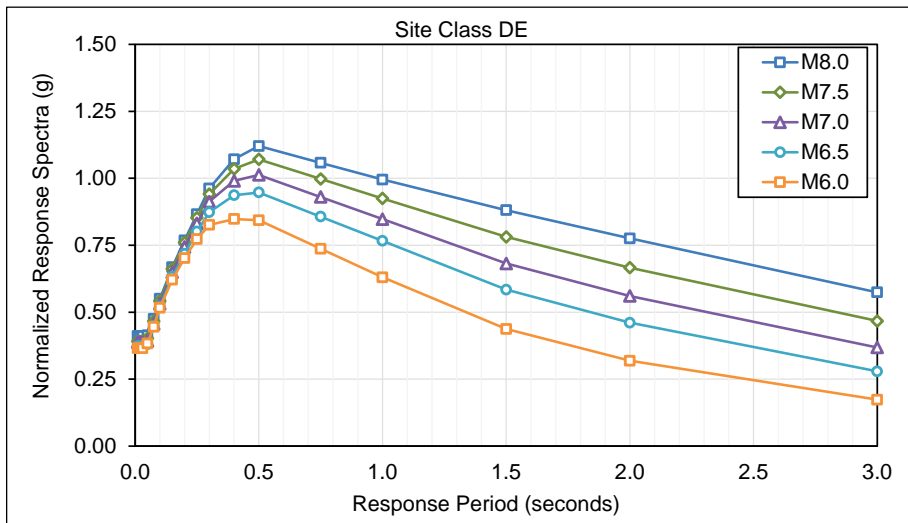
Figure 5.2-1 Plots of RSSPs for M6.0, M6.5, M7.0, M7.5, and M8.0; ground motion level S_5 = 1.5g and S_1 = 0.6g ; and Site Class BC (top), CD (middle), and DE (bottom).
