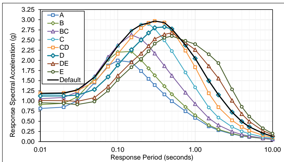
Figure E.1-12 Plots of probabilistic MCE_R multi-period response spectra (MPRS) derived from parameters S_s , S_l , T_L in accordance with the methods of Chapter 4, Oakland Site.
