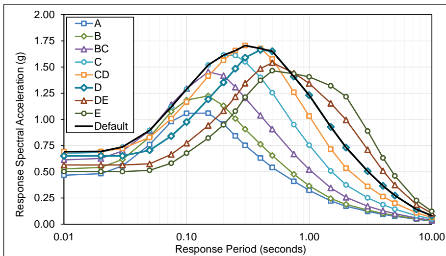
Figure E.2-6 Plots of deterministic MCE_R multi-period response spectra (MPRS) derived from parameters S_S and S_I in accordance with the methods of Chapter 5, Riverside Site.
