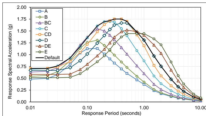
Figure 5.5-2 Plot of lower limit deterministic MPRS (Alternative 2).
