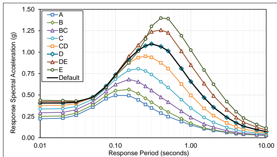
Figure E.3-15 Plots of MCE R multi-period response spectra (MPRS) derived from parameters S_s , S_l , T_L in accordance with the methods of Chapter 3, Sacramento Site.
