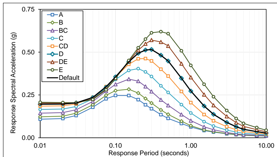
Figure E.3-27 Plots of MCE R multi-period response spectra (MPRS) derived from parameters S_s , S_l , T_L in accordance with the methods of Chapter 3, Boise Site.
