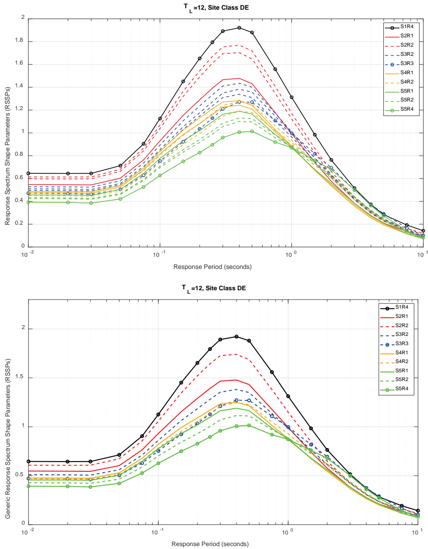
Figure 4.3-2 Plots of RSSPs (logarithmic horizontal axes) for and Site Class DE, for individual (S_s, R_{S/T}) bins (top), and for weighted averages of bins within (S_s, R_{S/T}) groups (bottom).
