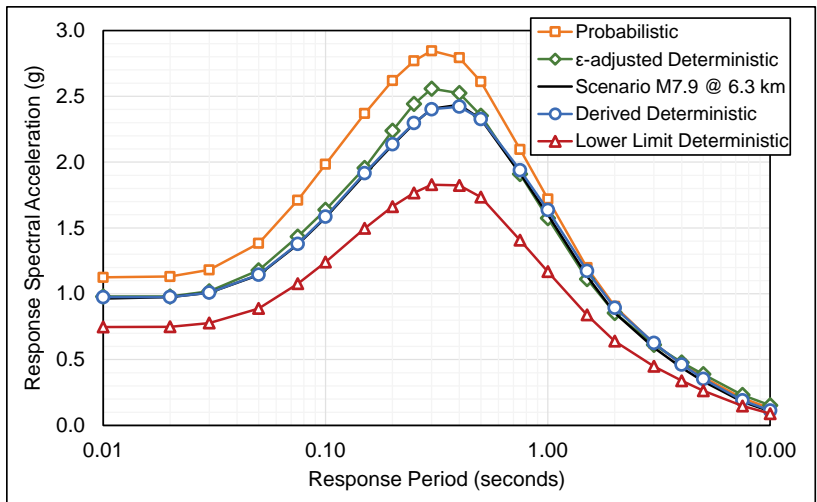
Figure 5.4-3 MCE_R Response Spectra, San Mateo Site, Site Class CD.
