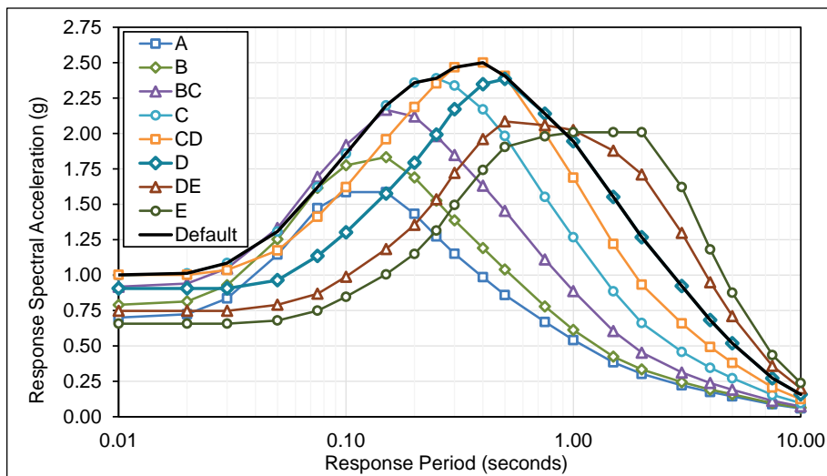
Figure E.2-22 Plots of deterministic MCE_R multi-period response spectra (MPRS) derived from parameters S_5 and S_1 in accordance with the methods of Chapter 5, Seattle Site.
