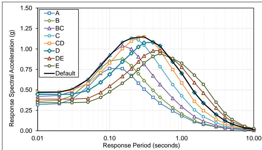
Figure C-4 Plots of deterministic response spectrum shape parameters (RSSPs) by site class, for ground motion level S_s = 1.5g/S_1 = 0.6g and earthquake magnitude 6.5.
