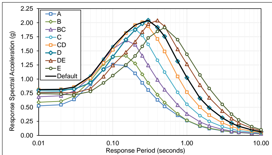
Figure E.3-32 Plots of MCE R multi-period response spectra (MPRS) derived from parameters S_s , S_l , T_L in accordance with the methods of Chapter 3, Charleston Site.
