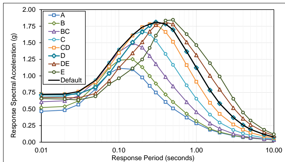
Figure E.3-5 Plots of MCE R multi-period response spectra (MPRS) derived from parameters S_s , S_l , T_L in accordance with the methods of Chapter 3, Irvine Site.
