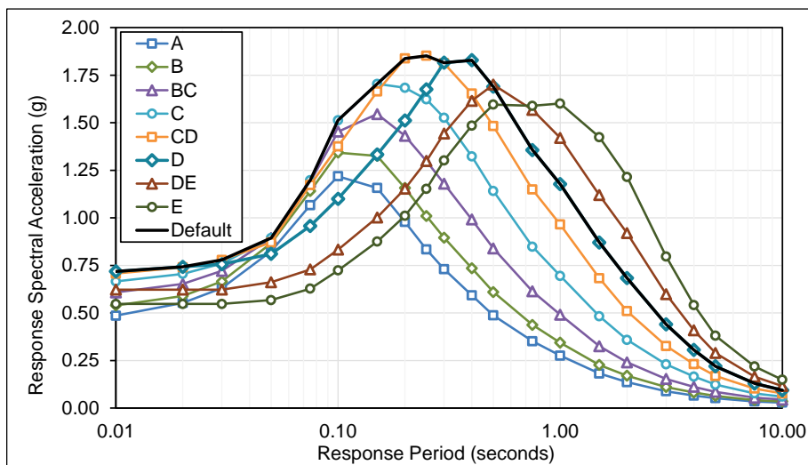
Figure E.3-24 Plots of MCE R multi-period response spectra (MPRS) derived from parameters S_s , S_l , T_L in accordance with the methods of Chapter 3, Everett Site.
