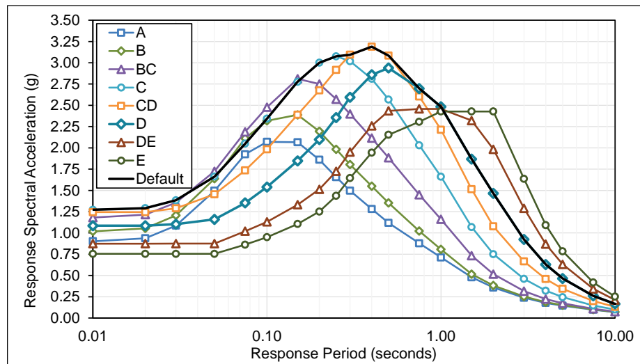
Figure E.3-21 Plots of MCE R multi-period response spectra (MPRS) derived from parameters S_s , S_l , T_L in accordance with the methods of Chapter 3, Santa Rosa Site.
