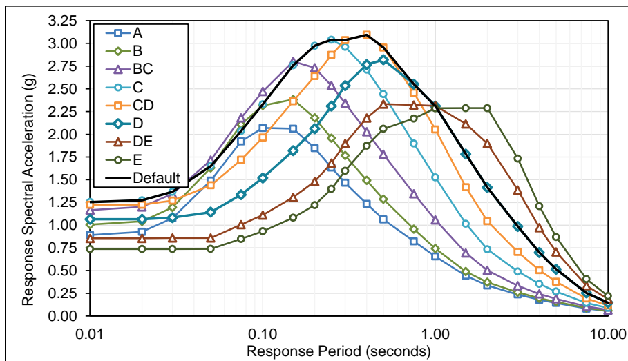
Figure E.2-2 Plots of deterministic MCE_R multi-period response spectra (MPRS) derived from parameters S_5 and S_1 in accordance with the methods of Chapter 5, Century City Site.
