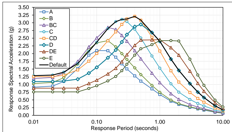
Figure E.3-7 Plots of MCE R multi-period response spectra (MPRS) derived from parameters S_s , S_l , T_L in accordance with the methods of Chapter 3, San Bernardino Site.
