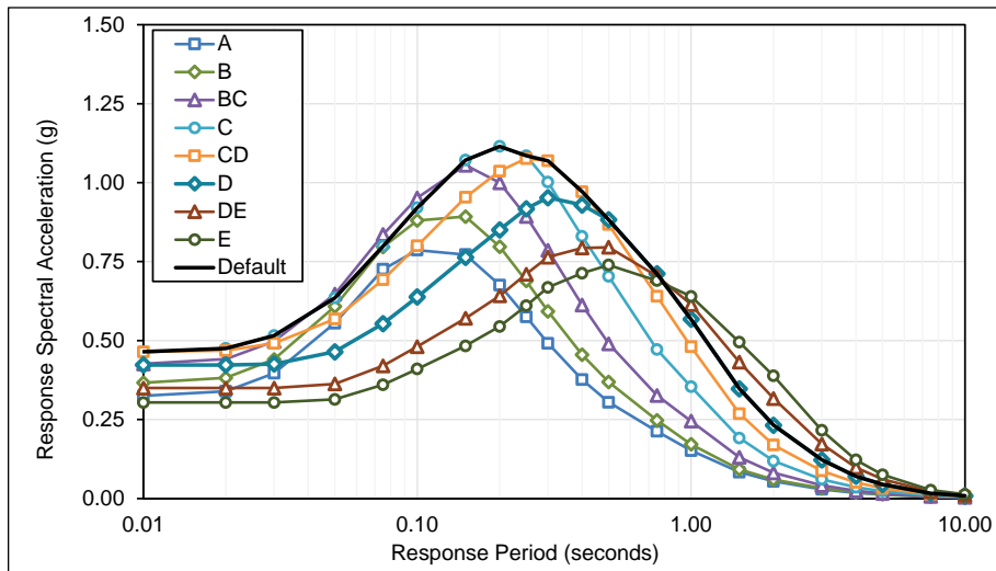
Figure C-10 Plots of deterministic response spectrum shape parameters (RSSPs) by site class, for ground motion level S_s = 2.0g/S_1 = 0.8g and earthquake magnitude 6.0.
