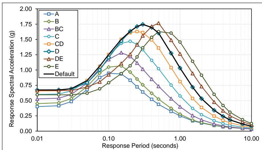
Figure E.3-8 Plots of MCE R multi-period response spectra (MPRS) derived from parameters S_s , S_l , T_L in accordance with the methods of Chapter 3, San Luis Obispo Site.
