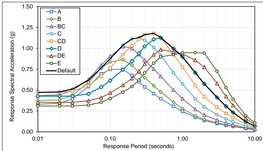
Figure C-6 Plots of deterministic response spectrum shape parameters (RSSPs) by site class, for ground motion level S_s = 2.0g/S_1 = 0.8g and earthquake magnitude 8.0.
