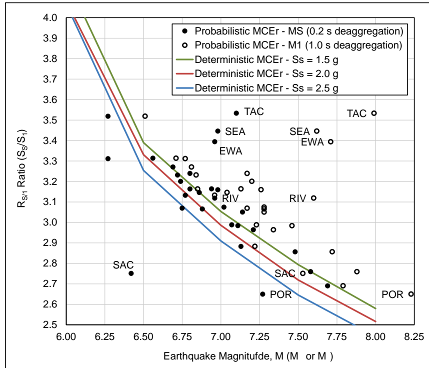
Figure 3.1-1 Values of the R_{S/I} ratio ( S_0.2/S_1 ) plotted as a function of earthquake magnitude obtained from deaggregation, where values of S_0.2 and S_1 are obtained from probabilistic MCE_R ground motions for example WUS sites, and underlying trends in the values R_{S/I} with earthquake magnitude, as determined from representative deterministic MCE_R ground motions.
