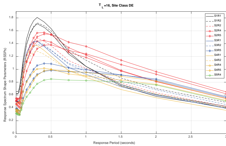
Figure 4.2-1 Plots of RSSPs for each (S_S, R_{S/1}) bin for T_L = 16 s; Site Class BC (top), Site Class CD (middle), and Site Class DE (bottom).
