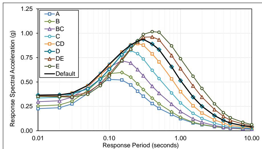
Figure E.3-29 Plots of MCE R multi-period response spectra (MPRS) derived from parameters S_s , S_l , T_L in accordance with the methods of Chapter 3, Las Vegas Site.
