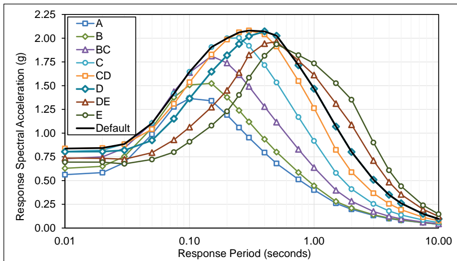
Figure E.3-26 Plots of MCE R multi-period response spectra (MPRS) derived from parameters S_s , S_l , T_L in accordance with the methods of Chapter 3, Salt Lake City Site.
