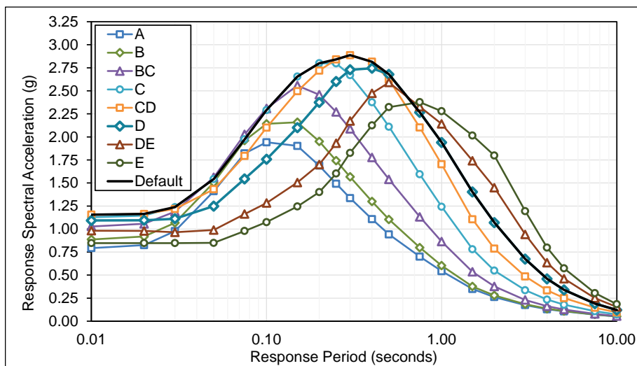
Figure E.3-10 Plots of MCE R multi-period response spectra (MPRS) derived from parameters S_s , S_l , T_L in accordance with the methods of Chapter 3, Santa Barbara Site.
