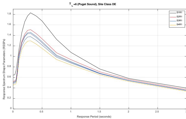
Figure 4.2-5 Plots of RSSPs for each ( S_S, R_{S/T} ) bin for T_L = 6 s inside Puget Sound region; Site Class BC (top), Site Class CD (middle), and Site Class DE (bottom).
