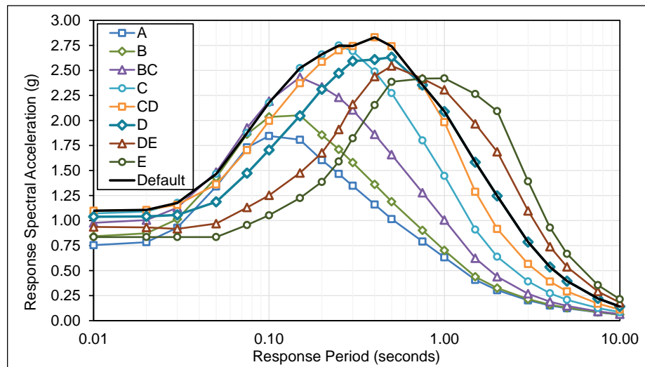
Figure E.3-11 Plots of MCE R multi-period response spectra (MPRS) derived from parameters S_s , S_l , T_L in accordance with the methods of Chapter 3, Ventura Site.
