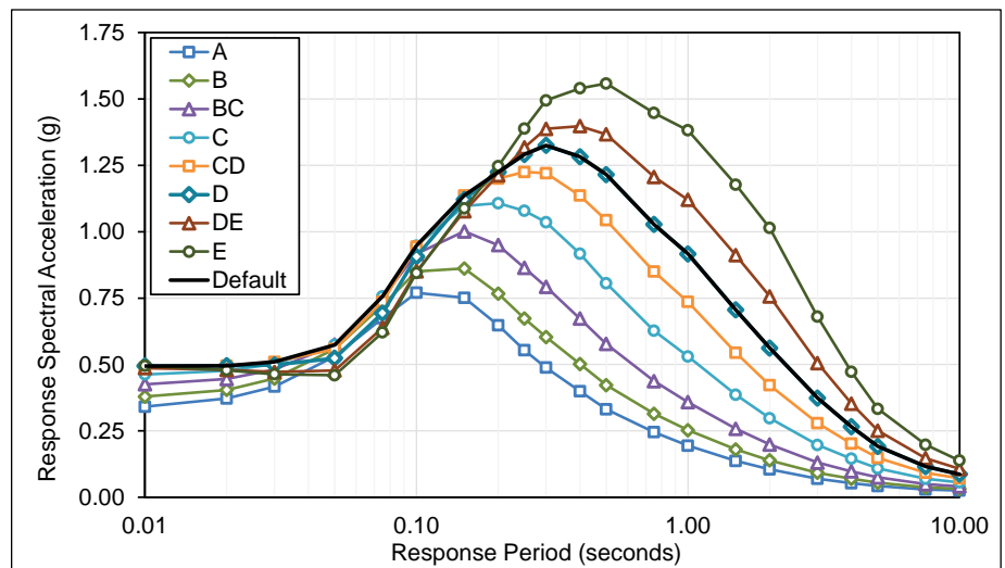
Figure E.1-25 Plots of probabilistic MCE_R multi-period response spectra (MPRS) derived from parameters S_s , S_l , T_L in accordance with the methods of Chapter 4, Portland Site.
