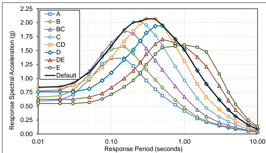
Figure E.2-24 Plots of deterministic MCE R multi-period response spectra (MPRS) derived from parameters S_5 and S_1 in accordance with the methods of Chapter 5, Everett Site.
