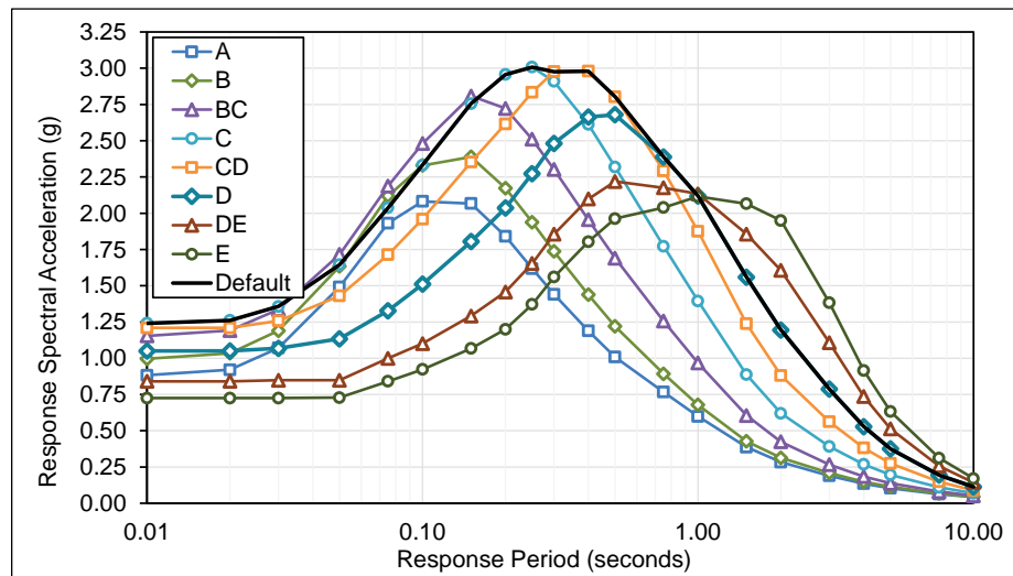
Figure E.3-13 Plots of MCE R multi-period response spectra (MPRS) derived from parameters S_s , S_l , T_L in accordance with the methods of Chapter 3, Concord Site.
