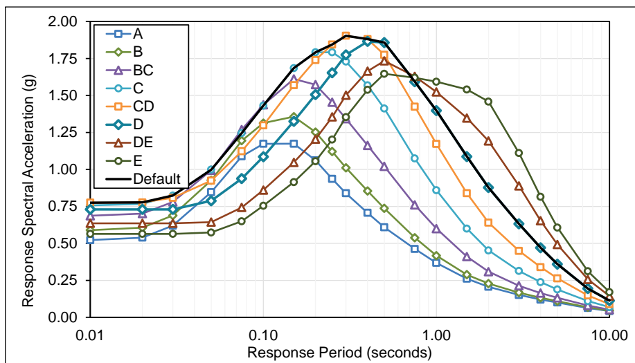
Figure E.3-16 Plots of MCE R multi-period response spectra (MPRS) derived from parameters S_s , S_l , T_L in accordance with the methods of Chapter 3, San Francisco Site.
