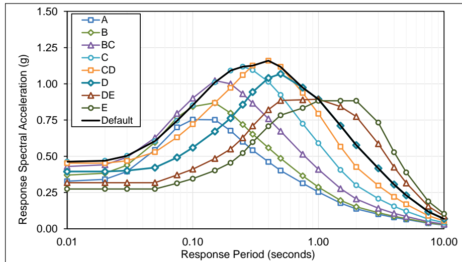
Figure C-11 Plots of deterministic response spectrum shape parameters (RSSPs) by site class, for ground motion level S_S = 2.5g/S_T = 1.0g and earthquake magnitude 8.0.
