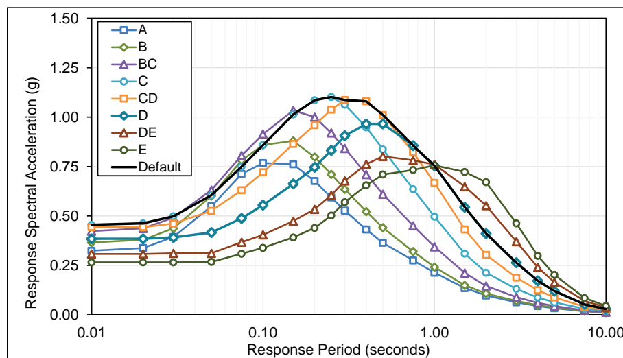
Figure C-13 Plots of deterministic response spectrum shape parameters (RSSPs) by site class, for ground motion level S_s = 2.5g/S_1 = 1.0g and earthquake magnitude 7.0.
