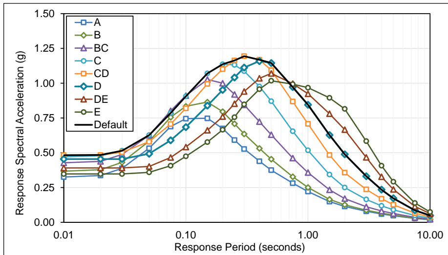
Figure C-2 Plots of deterministic response spectrum shape parameters (RSSPs) by site class, for ground motion level S_s = 1.5g/S_T = 0.6g and earthquake magnitude 7.5.
