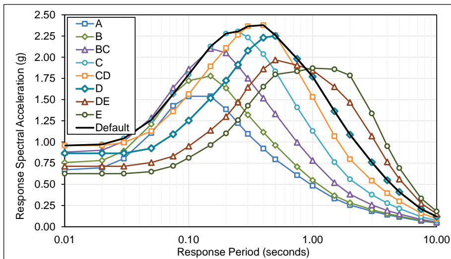
Figure E.2-12 Plots of deterministic MCE_R multi-period response spectra (MPRS) derived from parameters S_S and S_I in accordance with the methods of Chapter 5, Oakland Site.
