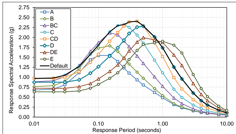
Figure E.3-3 Plots of MCE R multi-period response spectra (MPRS) derived from parameters S_s , S_l , T_L in accordance with the methods of Chapter 3, Northridge Site.
