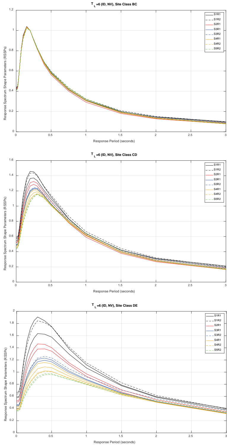
Figure 4.2-4 Plots of RSSPs for each ( S_S , R_{S/1} ) bin for T_L = 6 s outside Puget Sound region (i.e., Idaho and Nevada sites); Site Class BC (top), Site Class CD (middle), and Site Class DE (bottom).
