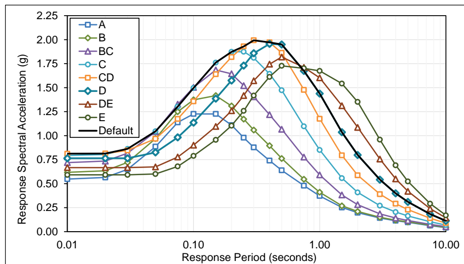
Figure E.3-19 Plots of MCE R multi-period response spectra (MPRS) derived from parameters S_s , S_l , T_L in accordance with the methods of Chapter 3, Santa Cruz Site.
