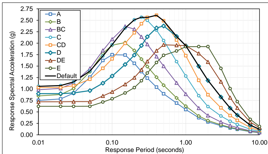
Figure E.2-20 Plots of deterministic MCE_R multi-period response spectra (MPRS) derived from parameters S_5 and S_1 in accordance with the methods of Chapter 5, Vallejo Site.
