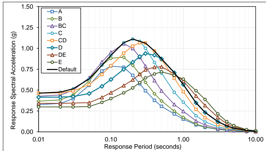
Figure C-15 Plots of deterministic response spectrum shape parameters (RSSPs) by site class, for ground motion level S_S = 2.5g/S_T = 1.0g and earthquake magnitude 6.0.
