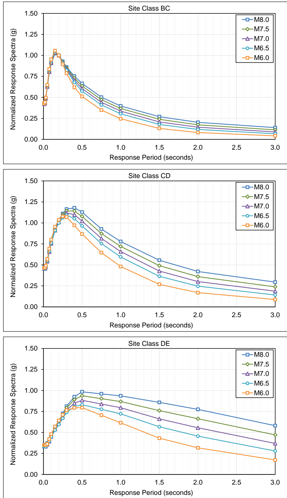
Figure 5.2-2 Plots of RSSPs for M6.0, M6.5, M7.0, M7.5, and M8.0; ground motion level S_5 = 2.0g and S_1 = 0.8g ; and Site Class BC (top), CD (middle), and DE (bottom).
