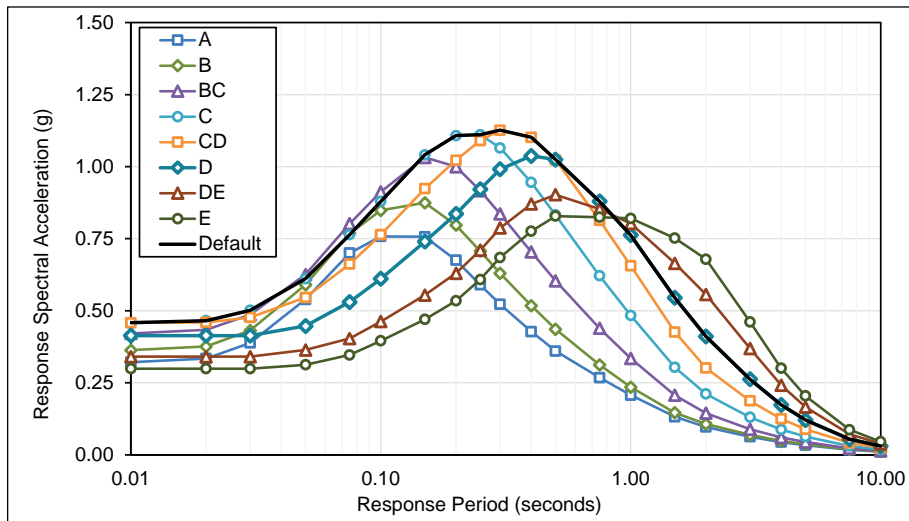
Figure C-8 Plots of deterministic response spectrum shape parameters (RSSPs) by site class, for ground motion level S_s = 2.0g/S_1 = 0.8g and earthquake magnitude 7.0.
