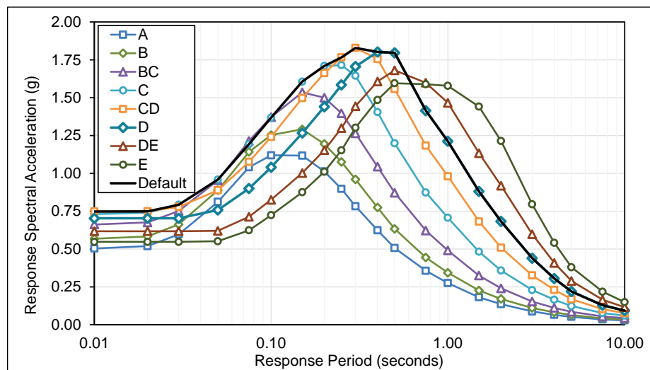
Figure E.3-23 Plots of MCE R multi-period response spectra (MPRS) derived from parameters S_s , S_l , T_L in accordance with the methods of Chapter 3, Tacoma Site.
