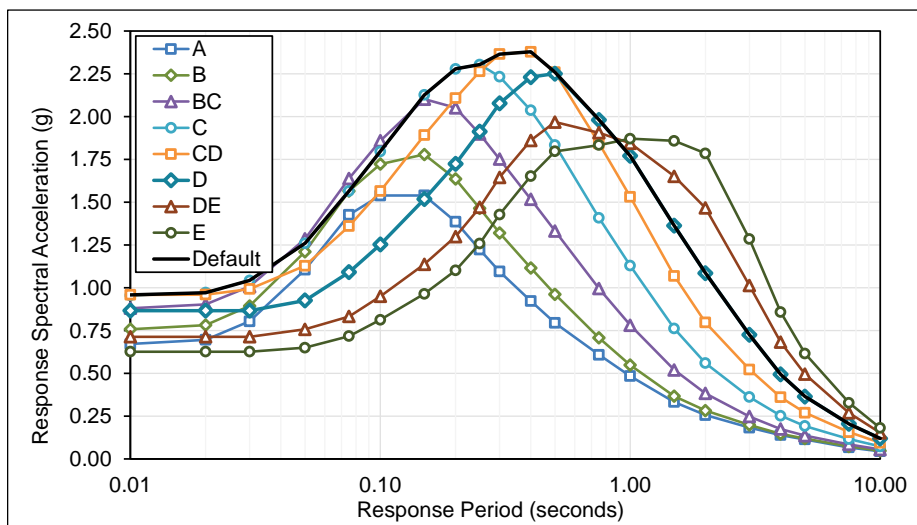
Figure E.3-12 Plots of MCE R multi-period response spectra (MPRS) derived from parameters S_s , S_l , T_L in accordance with the methods of Chapter 3, Oakland Site.
