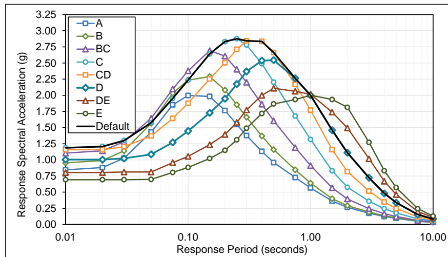
Figure E.2-1 Plots of deterministic MCE R multi-period response spectra (MPRS) derived from parameters S_5 and S_7 in accordance with the methods of Chapter 5, Los Angeles Site.
