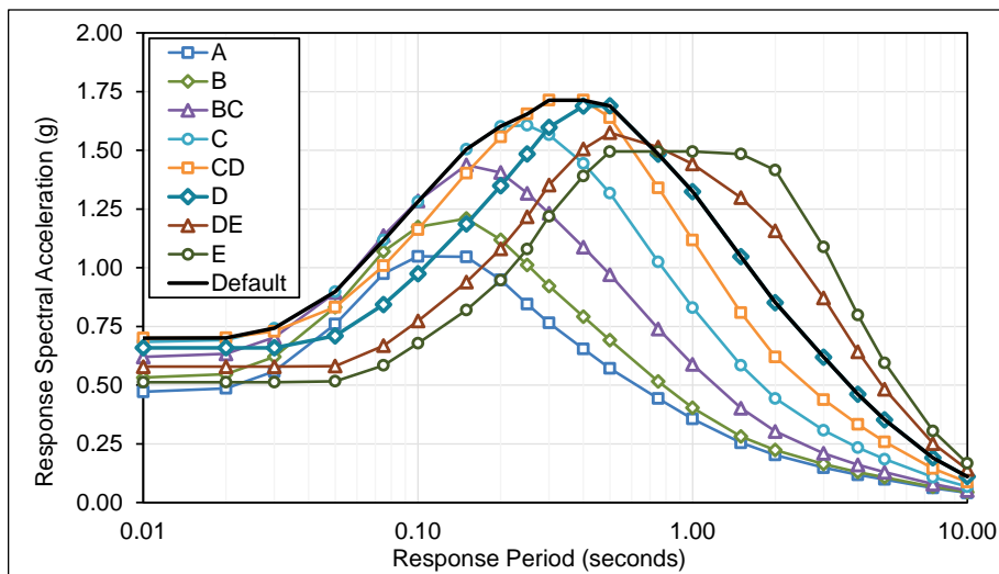
Figure E.2-18 Plots of deterministic MCE_R multi-period response spectra (MPRS) derived from parameters S_S and S_I in accordance with the methods of Chapter 5, San Jose Site.
