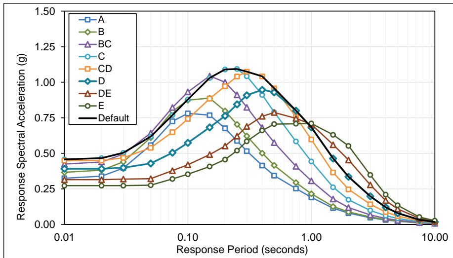
Figure C-14 Plots of deterministic response spectrum shape parameters (RSSPs) by site class, for ground motion level S_s = 2.5g/S_1 = 1.0g and earthquake magnitude 6.5.
