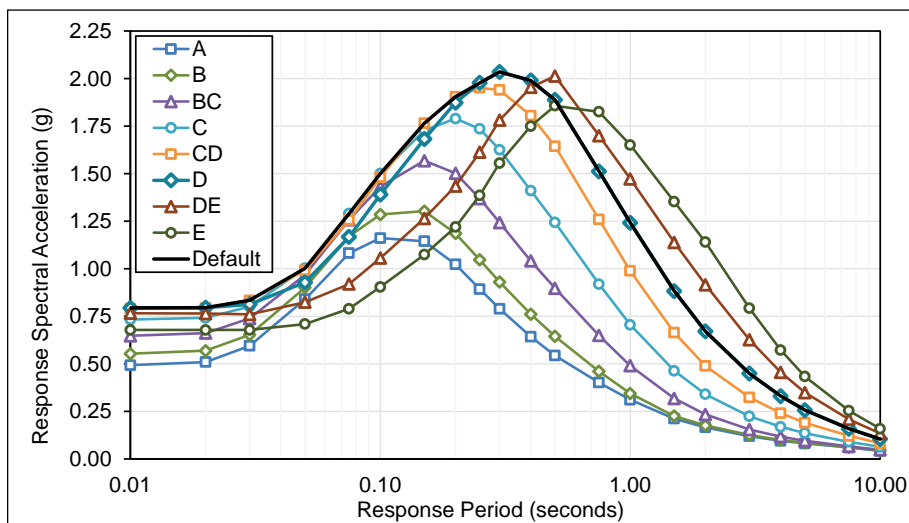
Figure E.3-14 Plots of MCE R multi-period response spectra (MPRS) derived from parameters S_s , S_l , T_L in accordance with the methods of Chapter 3, Monterey Site.
