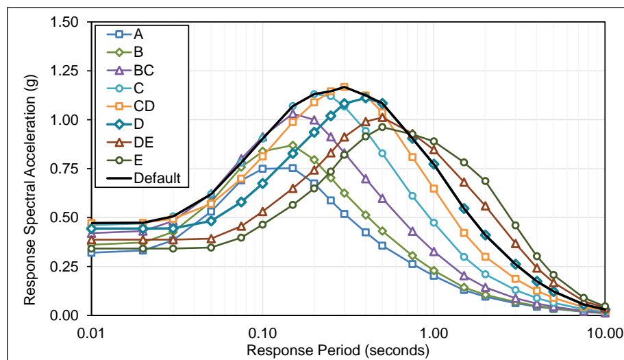
Figure C-3 Plots of deterministic response spectrum shape parameters (RSSPs) by site class, for ground motion level S_s = 1.5g/S_T = 0.6g and earthquake magnitude 7.0.
