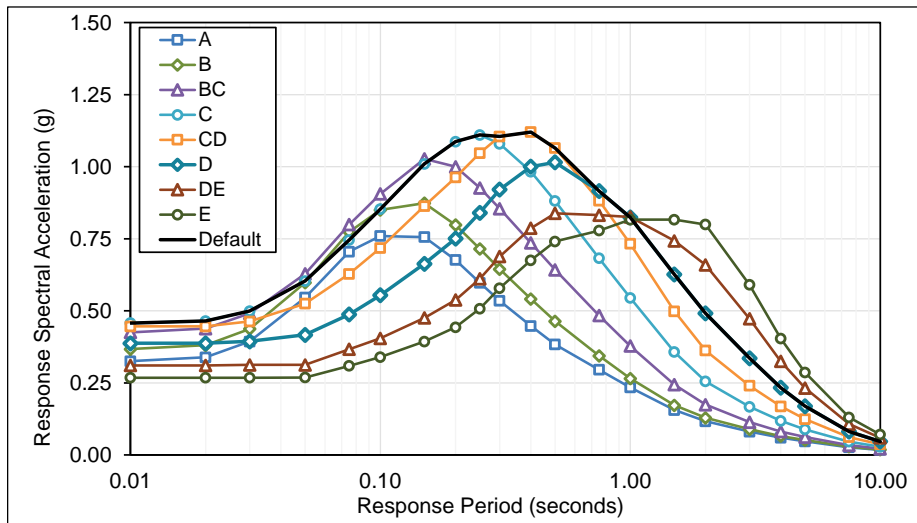
Figure C-12 Plots of deterministic response spectrum shape parameters (RSSPs) by site class, for ground motion level S_s = 2.5g/S_1 = 1.0g and earthquake magnitude 7.5.
