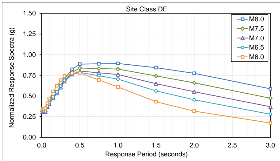
Figure 5.2-3 Plots of RSSPs for M6.0, M6.5, M7.0, M7.5, and M8.0; ground motion level S_5 = 2.5g and S_1 = 1.0g ; and Site Class BC (top), CD (middle), and DE (bottom).
