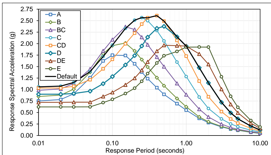
Figure E.3-20 Plots of MCE R multi-period response spectra (MPRS) derived from parameters S_s , S_l , T_L in accordance with the methods of Chapter 3, Vallejo Site.
