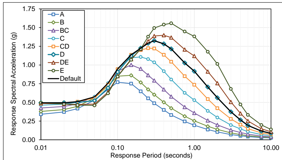
Figure E.3-25 Plots of MCE R multi-period response spectra (MPRS) derived from parameters S_s , S_l , T_L in accordance with the methods of Chapter 3, Portland Site.
