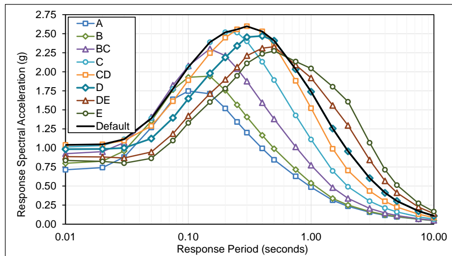
Figure E.1-3 Plots of probabilistic MCE_R multi-period response spectra (MPRS) derived from parameters S_s , S_l , T_L in accordance with the methods of Chapter 4, Northridge Site.
