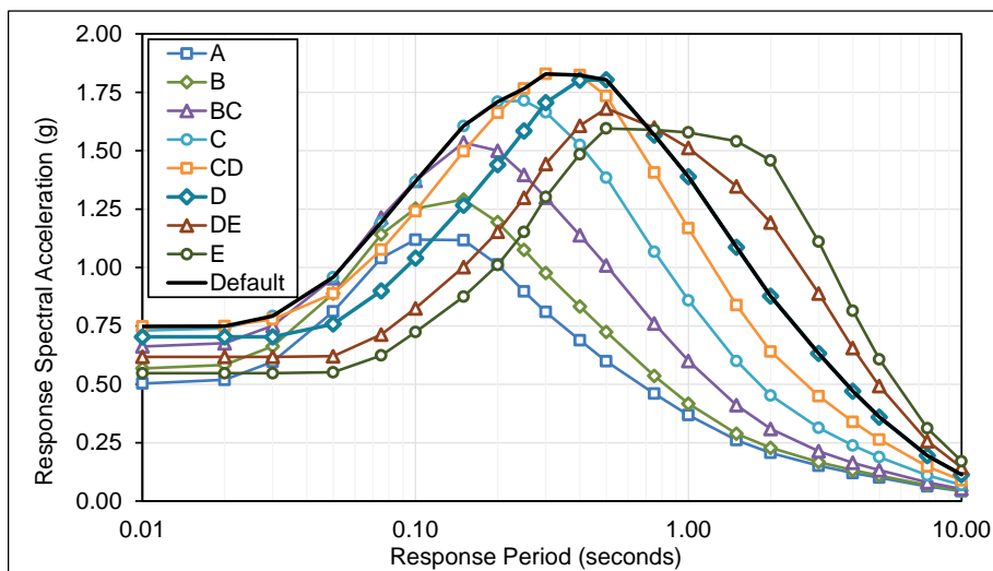
Figure E.3-18 Plots of MCE R multi-period response spectra (MPRS) derived from parameters S_s , S_l , T_L in accordance with the methods of Chapter 3, San Jose Site.
