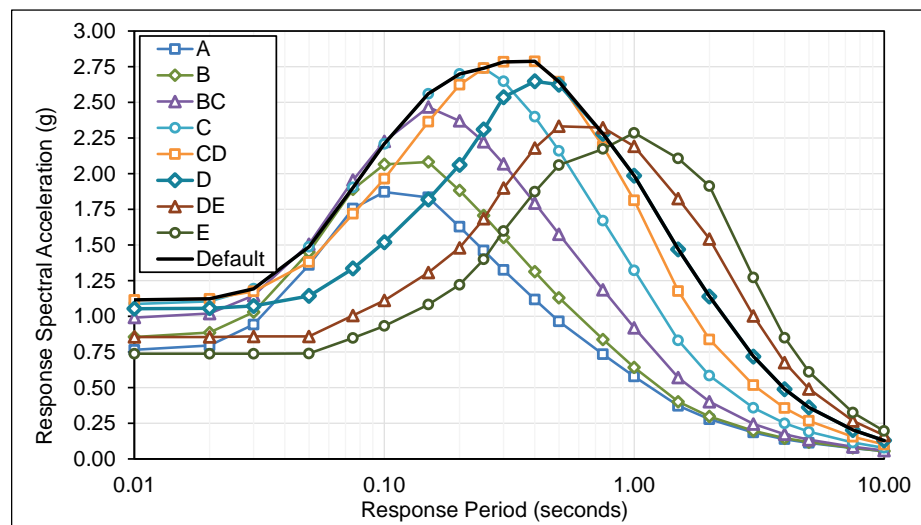
Figure E.3-2 Plots of MCE R multi-period response spectra (MPRS) derived from parameters S_s , S_l , T_L in accordance with the methods of Chapter 3, Century City Site.
