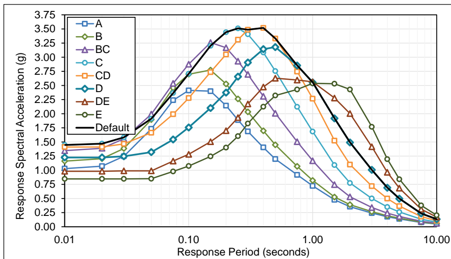
Figure E.2-10 Plots of deterministic MCE_R multi-period response spectra (MPRS) derived from parameters S_5 and S_1 in accordance with the methods of Chapter 5, Santa Barbara Site.
