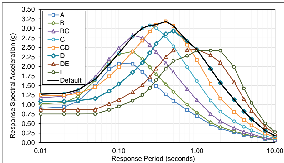
Figure E.2-4 Plots of deterministic MCE_R multi-period response spectra (MPRS) derived from parameters S_5 and S_1 in accordance with the methods of Chapter 5, Long Beach Site.
