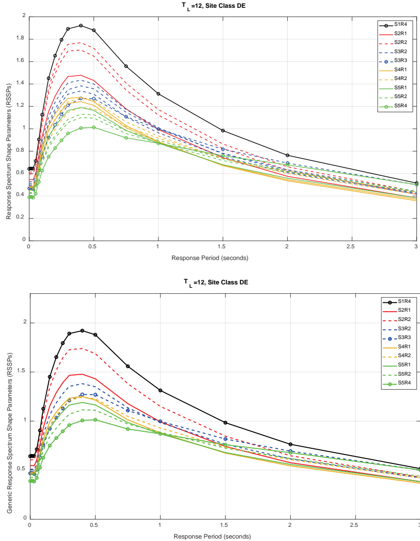
Figure 4.3-1 Plots of RSSPs (linear horizontal axes) for T_L = 12 s and Site Class DE, for individual ( S_S, R_{S/I} ) bins (top), and for weighted averages of bins within ( S_S, R_{S/I} ) groups (bottom).
