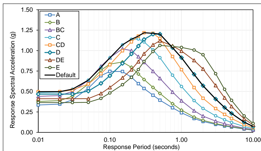
Figure C-1 Plots of deterministic response spectrum shape parameters (RSSPs) by site class, for ground motion level S_S = 1.5g/S_T = 0.6g and earthquake magnitude 8.0.
