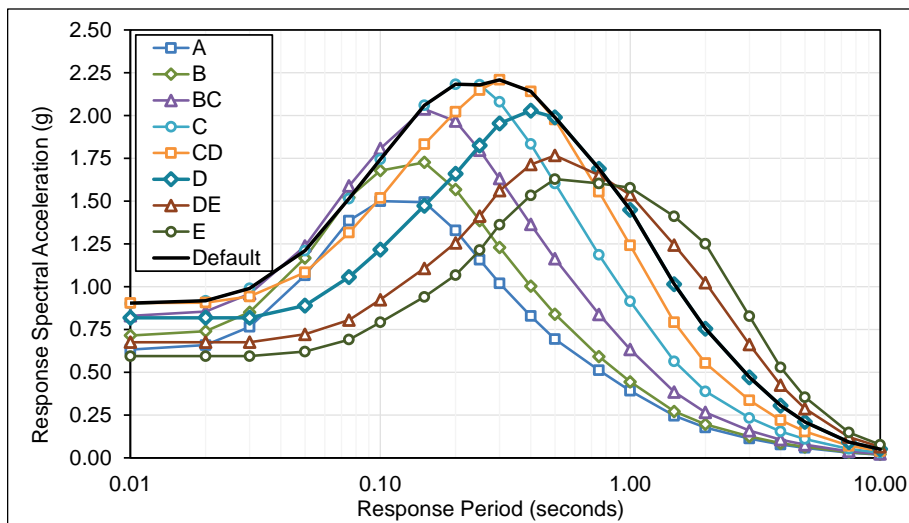
Figure E.2-8 Plots of deterministic MCE_R multi-period response spectra (MPRS) derived from parameters S_S and S_I in accordance with the methods of Chapter 5, San Luis Obispo Site.
