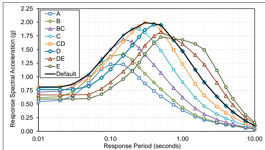
Figure E.2-19 Plots of deterministic MCE_R multi-period response spectra (MPRS) derived from parameters S_S and S_I in accordance with the methods of Chapter 5, Santa Cruz Site.
