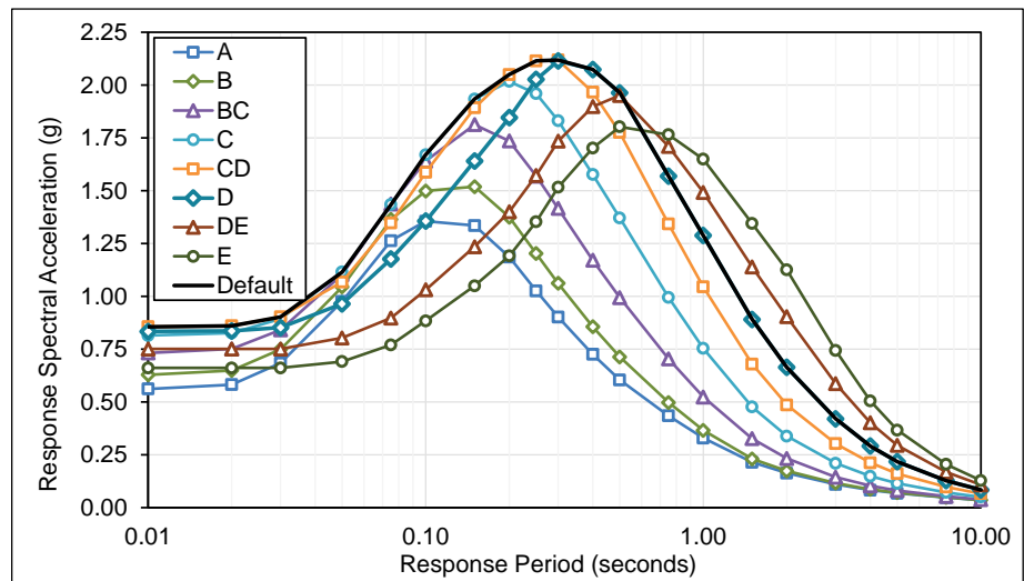
Figure E.3-9 Plots of MCE R multi-period response spectra (MPRS) derived from parameters S_s , S_l , T_L in accordance with the methods of Chapter 3, San Diego Site.
