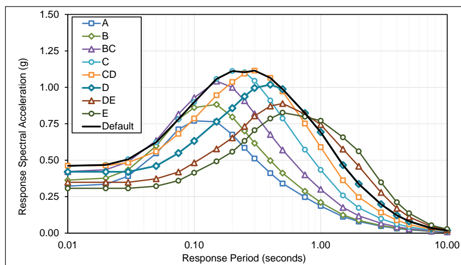
Figure C-9 Plots of deterministic response spectrum shape parameters (RSSPs) by site class, for ground motion level S_S = 2.0g/S_T = 0.8g and earthquake magnitude 6.5.
