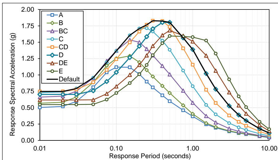
Figure E.3-6 Plots of MCE R multi-period response spectra (MPRS) derived from parameters S_s , S_l , T_L in accordance with the methods of Chapter 3, Riverside Site.
