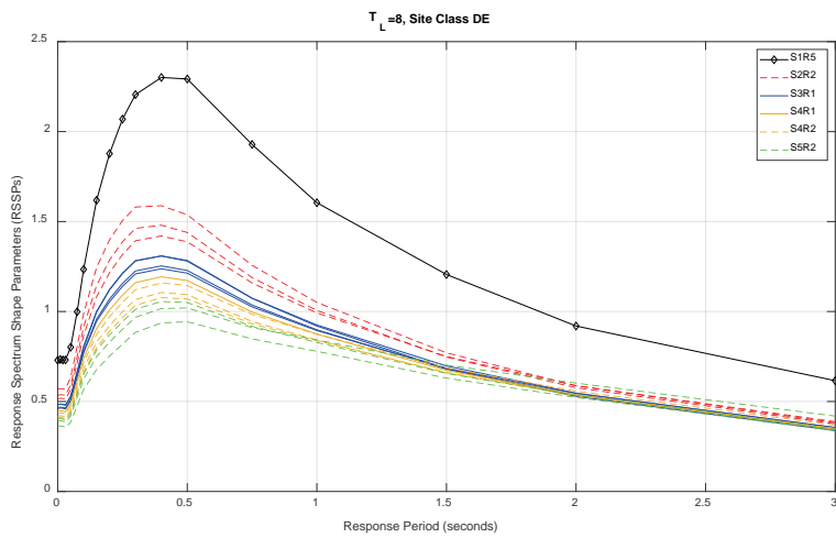
Figure 4.2-3 Plots of RSSPs for each ( S_S , R_{S/1} ) bin for T_L = 8 s; Site Class BC (top), Site Class CD (middle), and Site Class DE (bottom).
