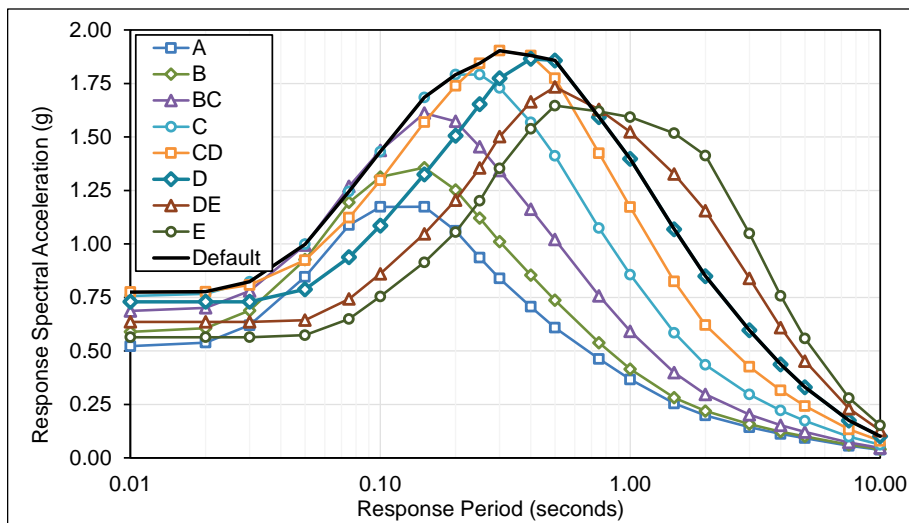
Figure E.2-16 Plots of deterministic MCE_R multi-period response spectra (MPRS) derived from parameters S_S and S_I in accordance with the methods of Chapter 5, San Francisco Site.
