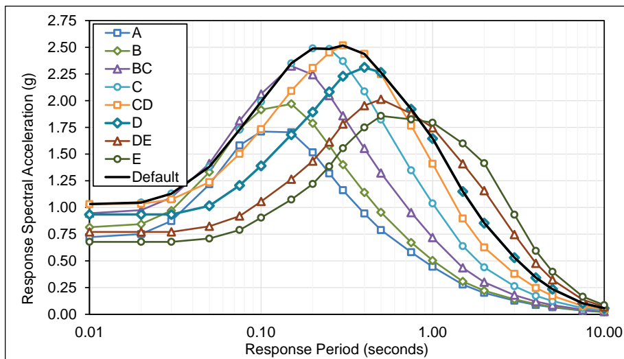
Figure E.2-14 Plots of deterministic MCE_R multi-period response spectra (MPRS) derived from parameters S_5 and S_1 in accordance with the methods of Chapter 5, Monterey Site.
