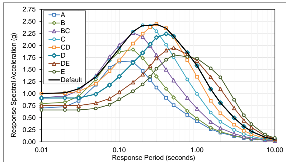
Figure E.2-9 Plots of deterministic MCE_R multi-period response spectra (MPRS) derived from parameters S_S and S_I in accordance with the methods of Chapter 5, San Diego Site.
